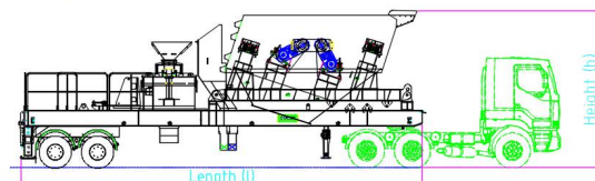
Transport Mode Side view - with Screen
