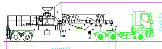
Transport Mode Side view - without Screen
